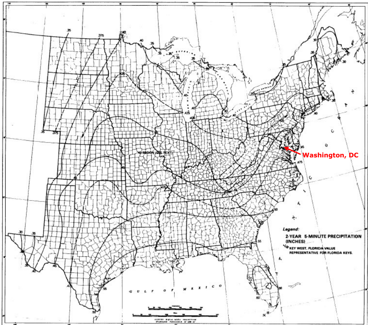
Figure 1. 2-Year, 5-Minute Precipitation (inches) – Adjusted to Partial-Duration Series (Source: NOAA Technical Memorandum NWS HYDRO-35)
