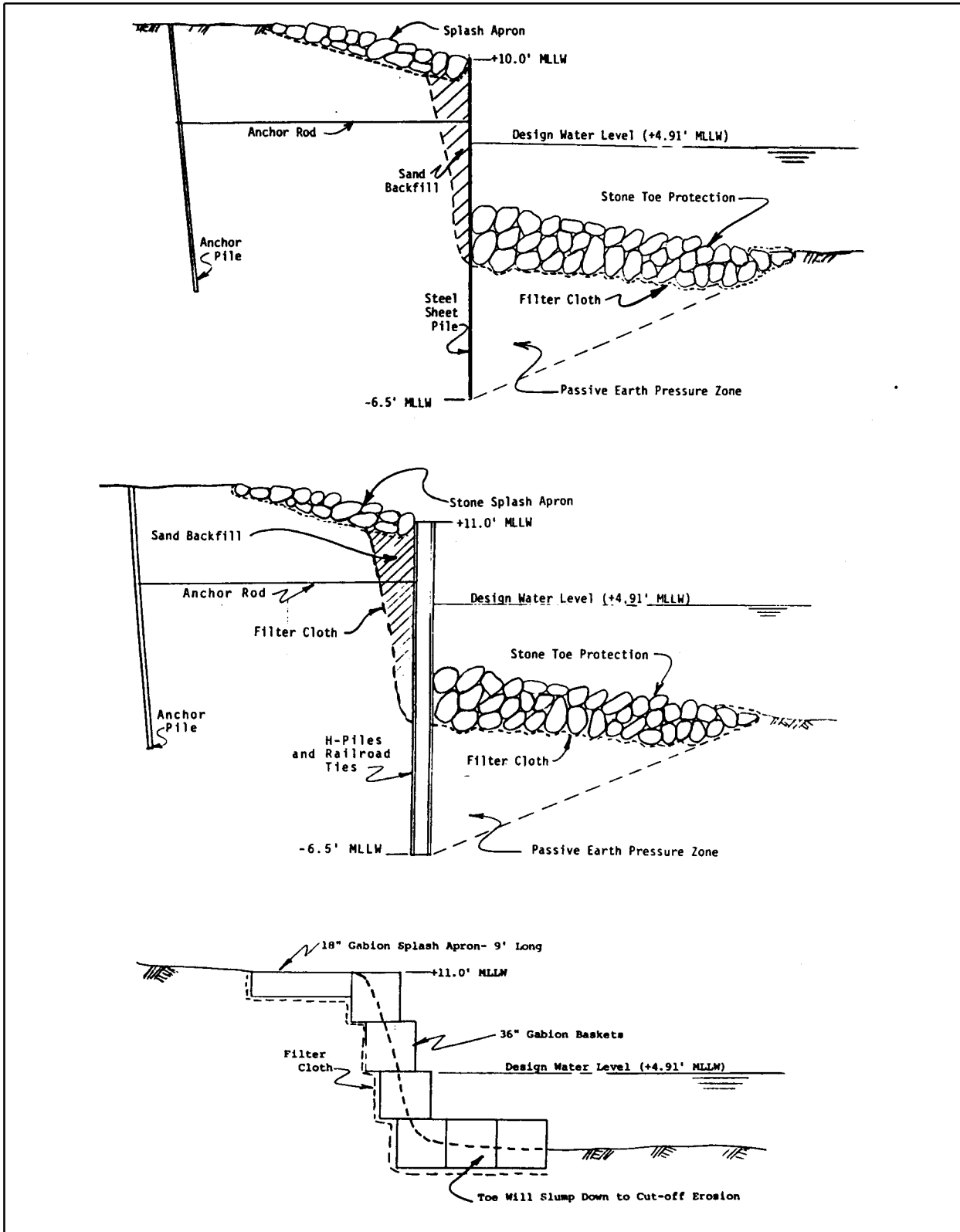
Figure E-3. Bulkhead section alternatives
