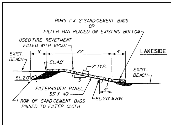
Figure B-47. Tire mattress revetment cross section
