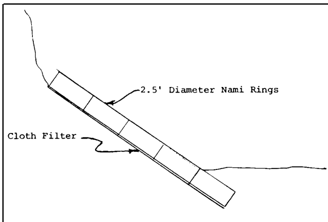
Figure B-20. Nami Ring revetment cross section
