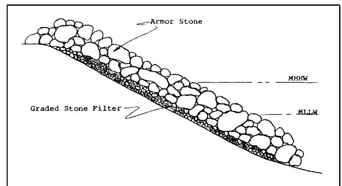
Figure B-2. Quarrystone revetment cross section
