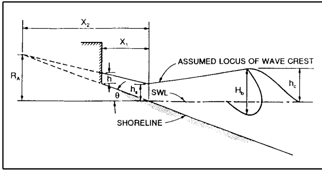
Figure 2-10. Wave pressure from broken waves
