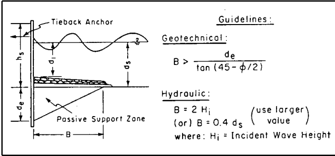
Figure 2-6. Toe aprons for sheet-pile bulkheads
