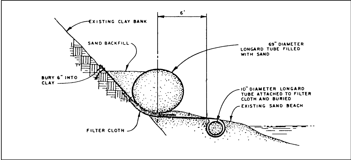
Figure D-26. Longard tube bulkhead cross section
