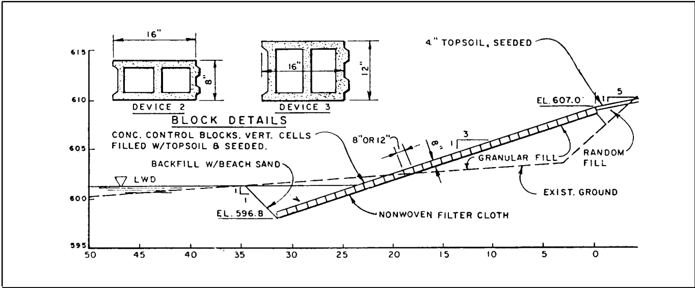
Figure B-25. Concrete control block revetment cross section
