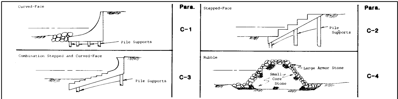
Figure 4.2. Summary of seawall alternatives
