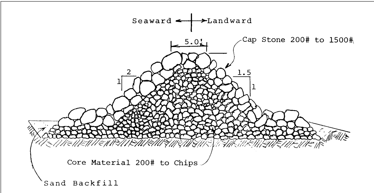
Figure C-8. Rubble-mound seawall cross section
