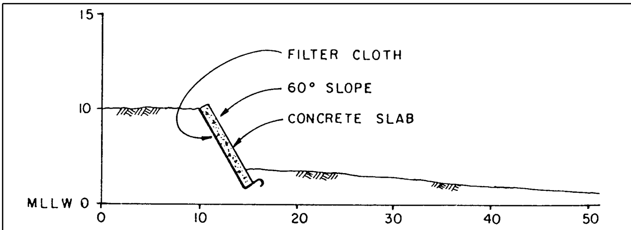
Figure B-43. Concrete slab revetment B-26
