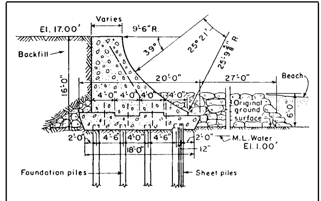
Figure C-2. Curved-face seawall cross section
