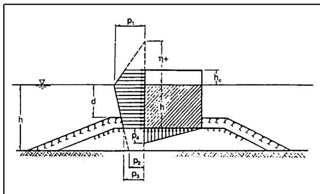
Figure 2-9. Breaking wave pressure on a vertical wall
