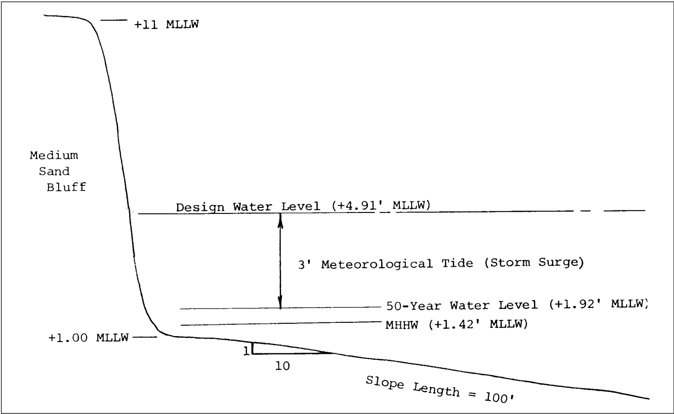
Figure E-1. Site conditions for sample problem
