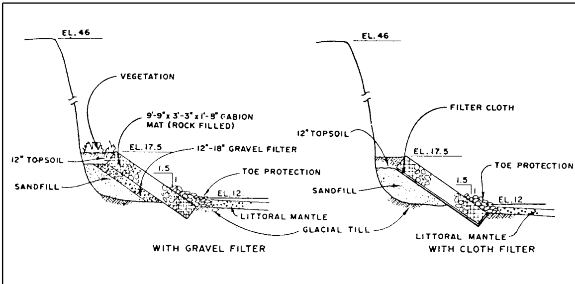
Figure B-37. Gabion revetment cross section
