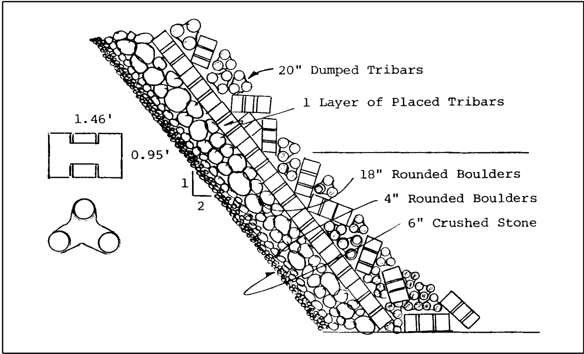
Figure B-11. Concrete tribar revetment cross section
