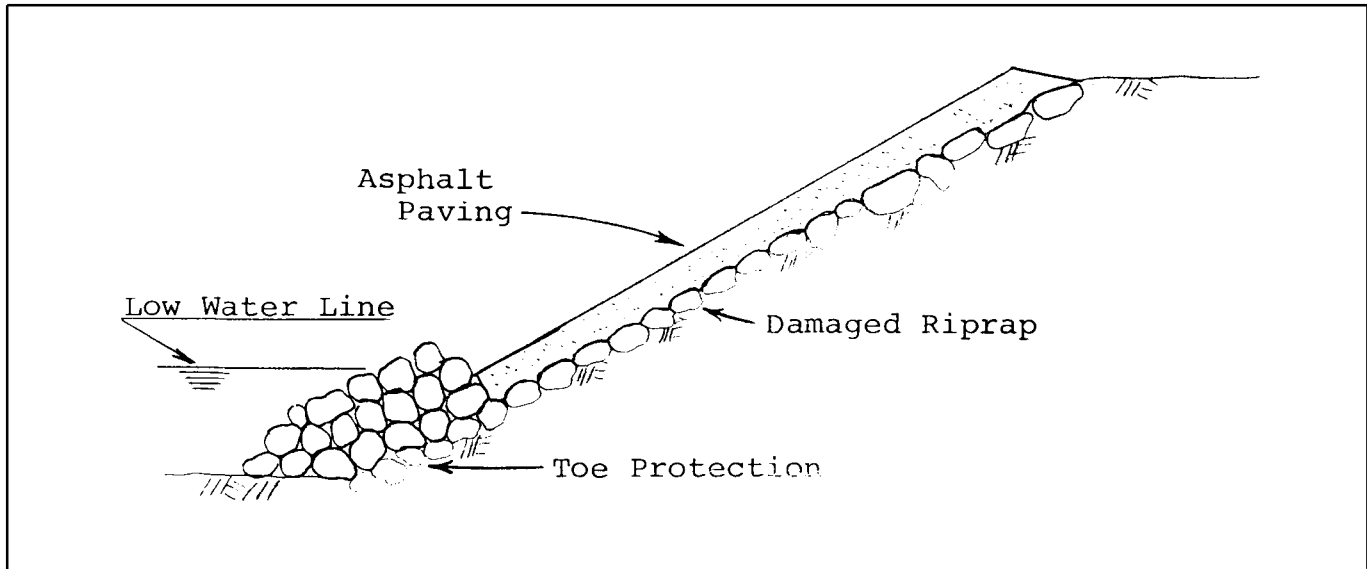
Figure B-9. Asphaltic concrete revetment cross section
