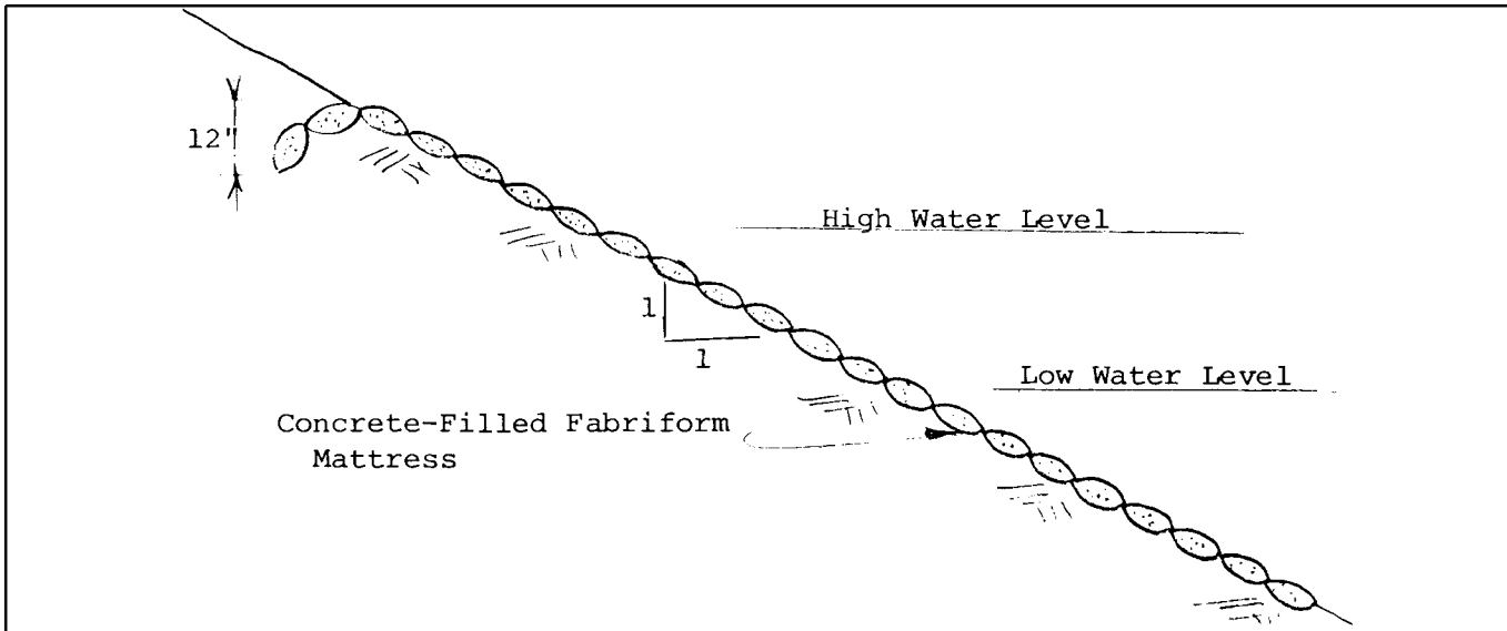
Figure B-33. Fabriform revetment cross section
