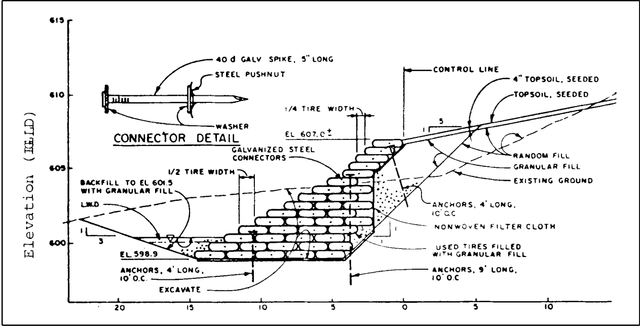
Figure D-22. Stacked rubber tire bulkhead cross section
