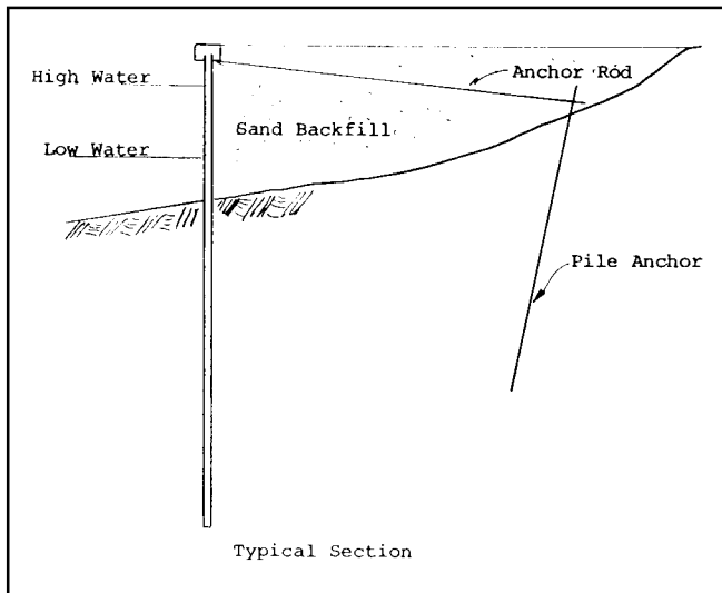
Figure D-5. Aluminum sheet-pile bulkhead cross section
