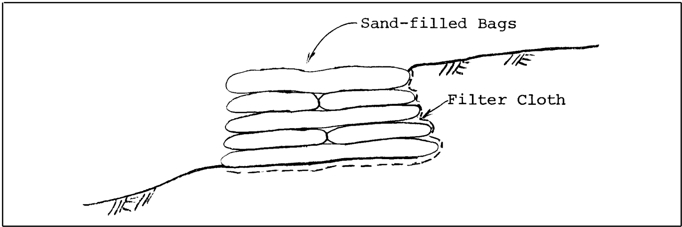
Figure D-27. Stacked bag bulkhead cross section
