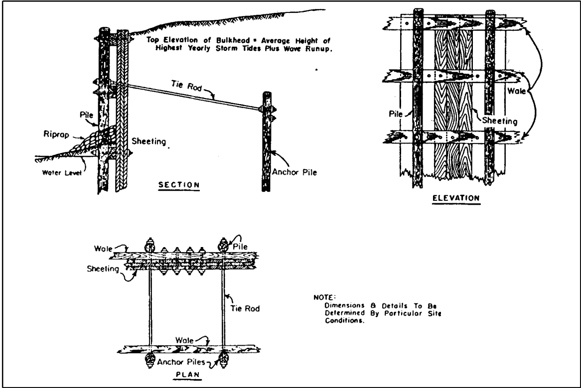
Figure D-4. Construction details of timber sheet-pile bulkhead
