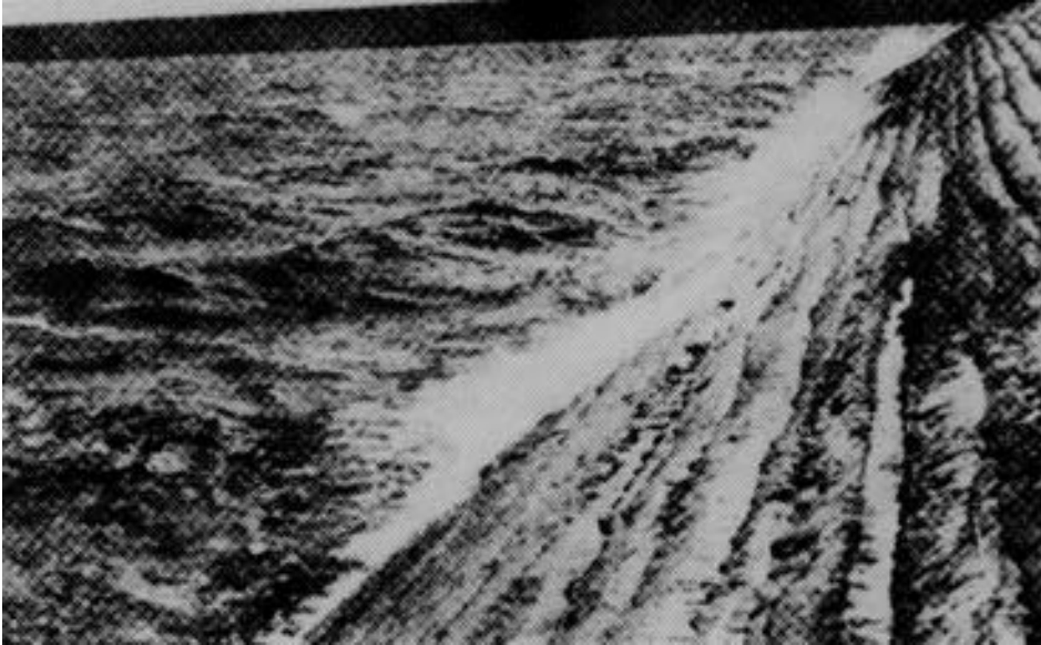
Figure B-44. Soil cement revetment, Bonny Dam, CO
