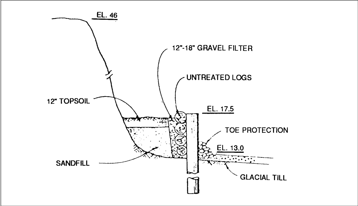
Figure D-15. Untreated log bulkhead cross section
