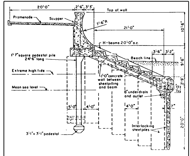
Figure C-6. Combination stepped- and curved-face seawall cross section
