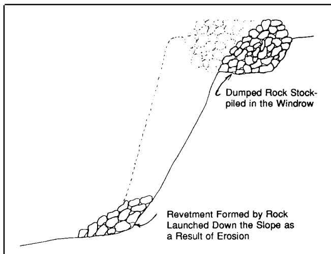
Figure B-49. Windrow revetment
