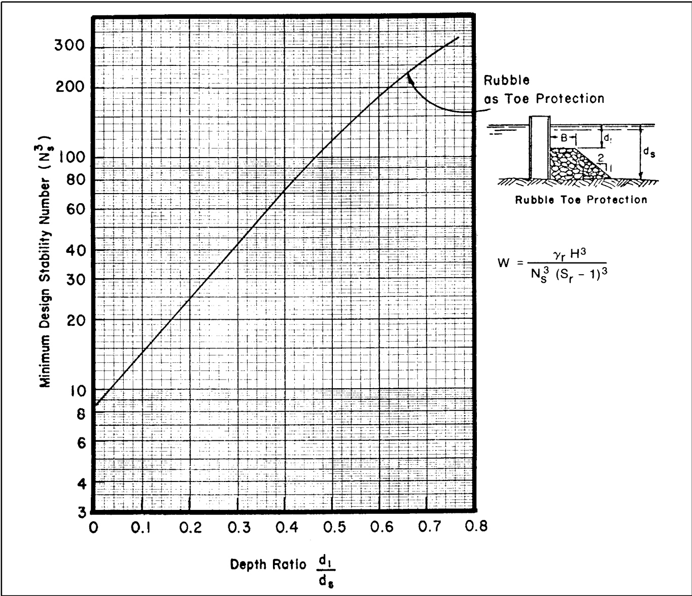
Figure 2-7. Value N_s , toe protection design for vertical walls (from Brebner and Donnelly 1962)
