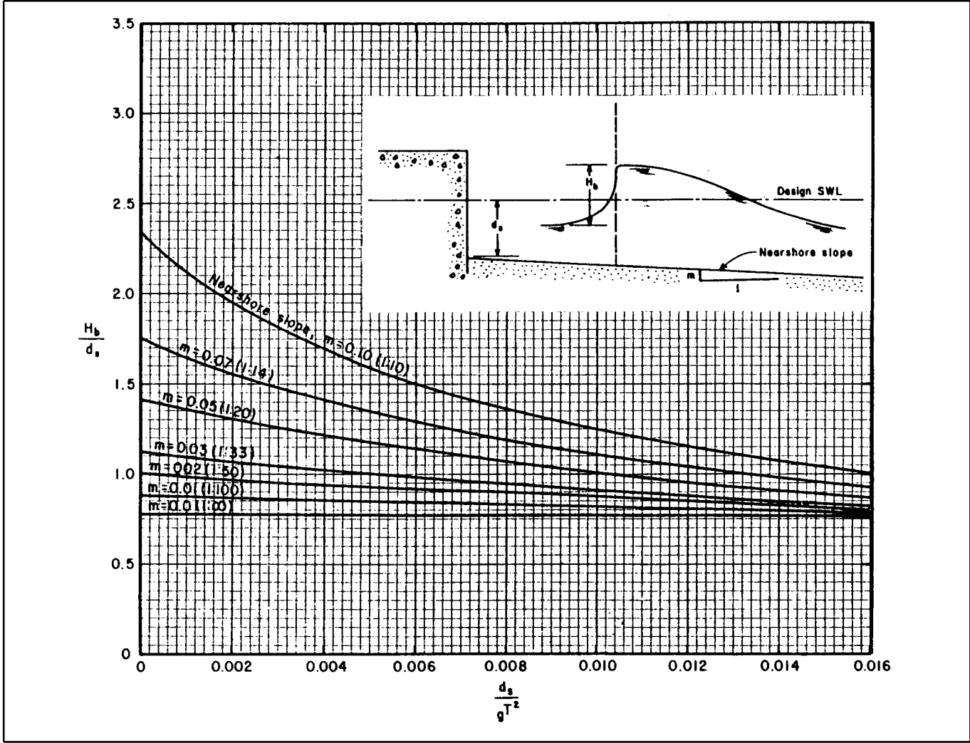
Figure 2-2. Design breaker height
