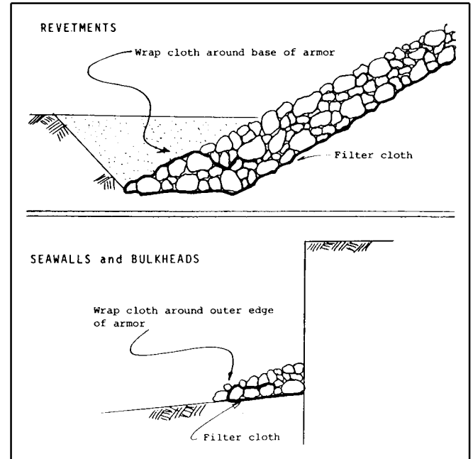
Figure 2-8. Use of filter cloth under revetment and toe protection stone
