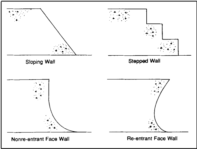
Figure 4-1. Typical concrete seawall sections
