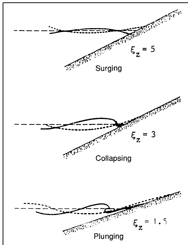
Figure 2-3. Surf parameter and breaking wave types
