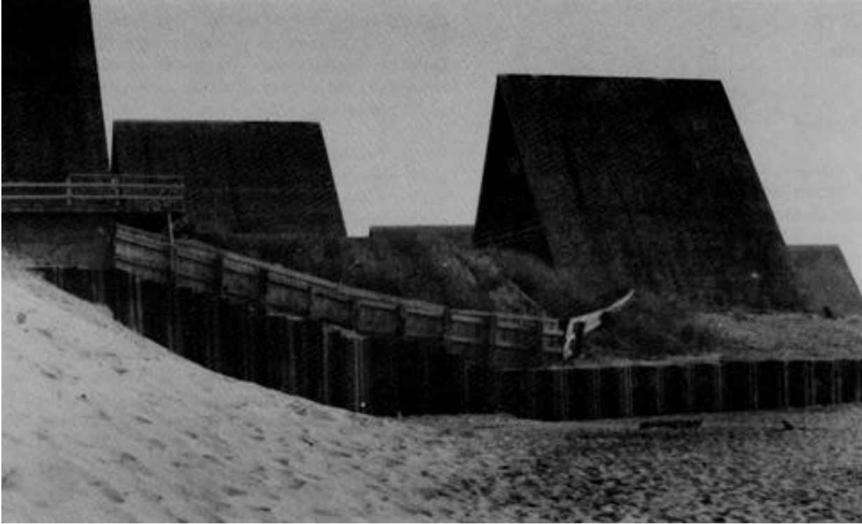
Figure D-1. Sheet-pile bulkhead, Lincoln Township, MI
