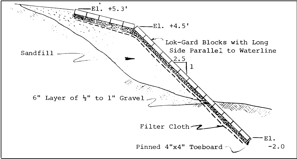
Figure B-29. Lok-Gard block revetment cross section
